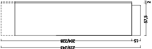
COLONNE FRIGO FRIDGE COLUMNS
