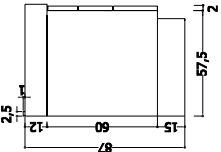
BASI H 75 PER TOP H 12 BASE UNITS H 75 FOR TOP H 12
